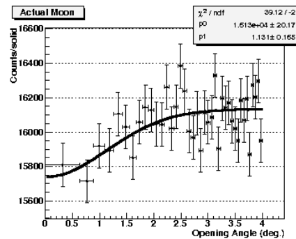
Figure 3: Variation of shower rate with opening angle centered on the Moon. Each bin has same solid angle. Angular resolution was calculated to be 1.13^\circ with the shower size of \log_{10}(\text{Size}) \geq 3.2 .
